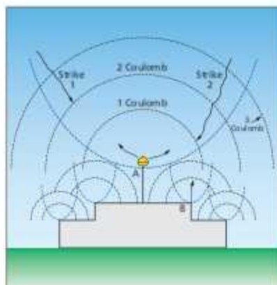
The Collection Volume Method defines the lightning “capture volume” of potential strike points on a structure. This method is used in conjunction with the ERITECH® SYSTEM 3000 lightning protection system but is equally applicable for the placement of conventional terminals.
